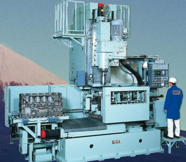
Cylinder block machining Vertical Boring Machine
